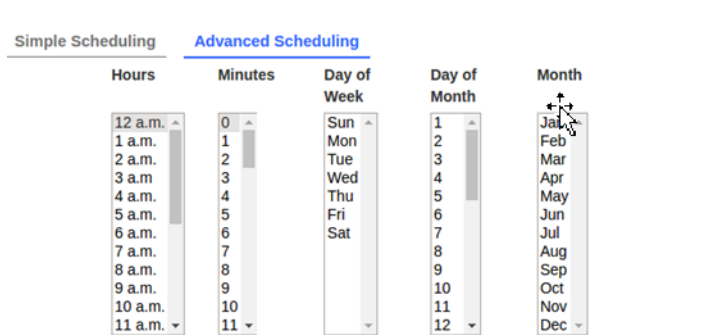
Figure 6–11 Schedule Frequency
