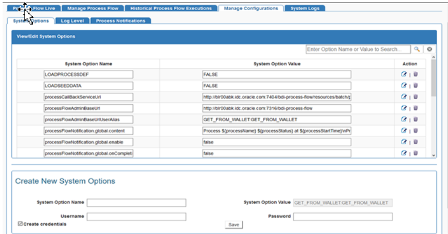
Figure 5–15 Create Credentials
