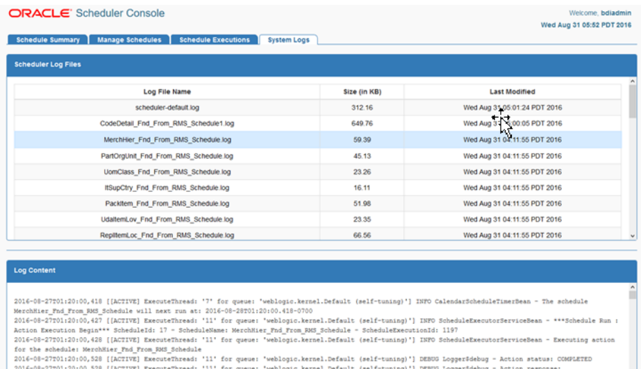
Figure 6–22 System Logs
