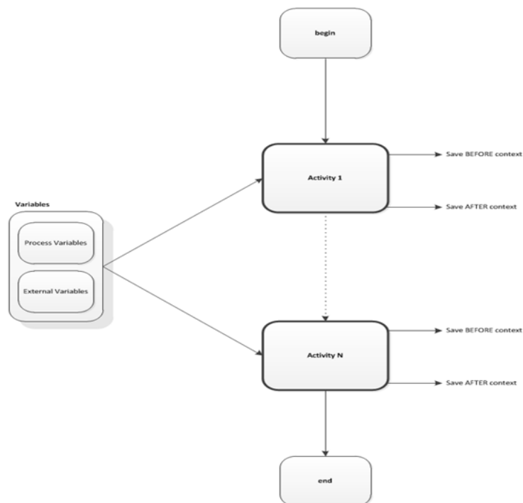
Figure 5-1 Process Flow
